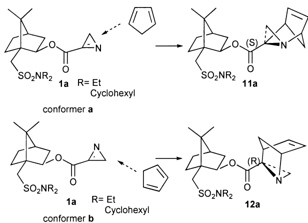
Fig. 4 Approach of cyclopentadiene to the less hindered face of two conformations of the azirine 1a .
